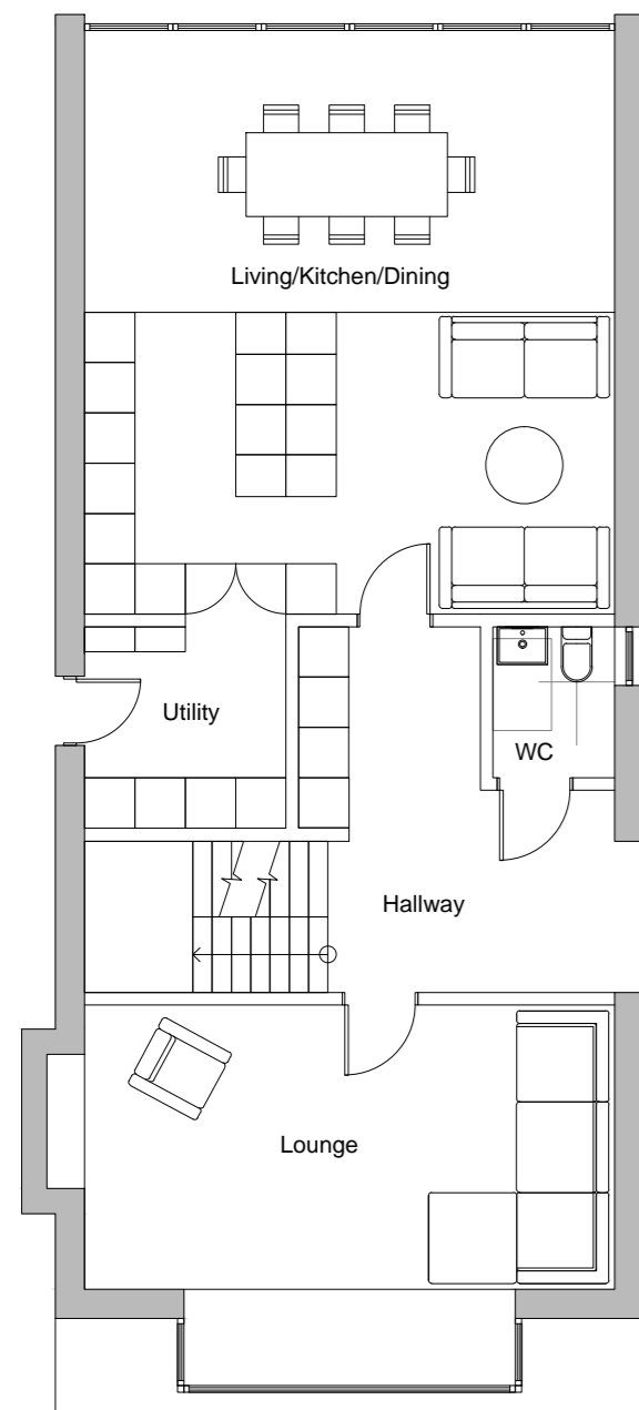
House 1 Proposed Ground Floor Plan 1:100
