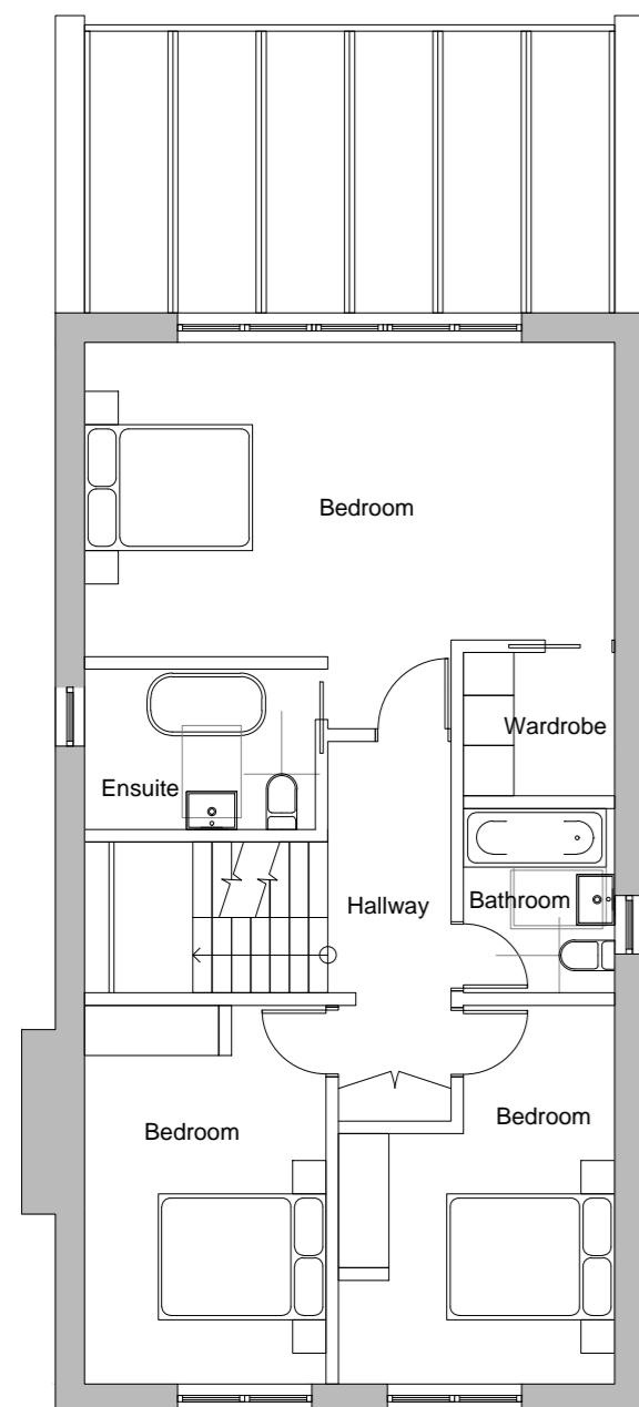
House 1 Proposed First Floor Plan 1:100
